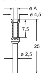
CCF and CCM
