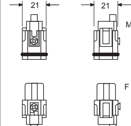
contacts side (front view)
