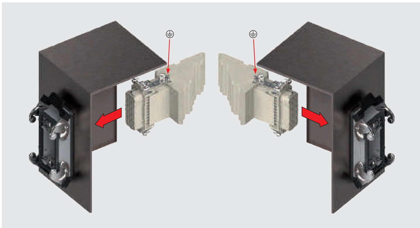
Figure 3 (left mounting)
