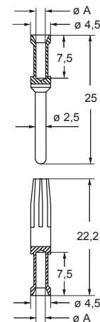
CCF and CCM contacts
