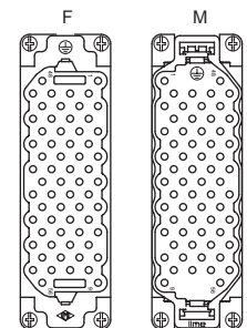
contacts side (front view)
