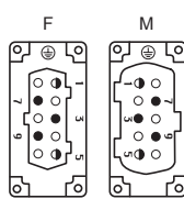
contacts side (front view)
