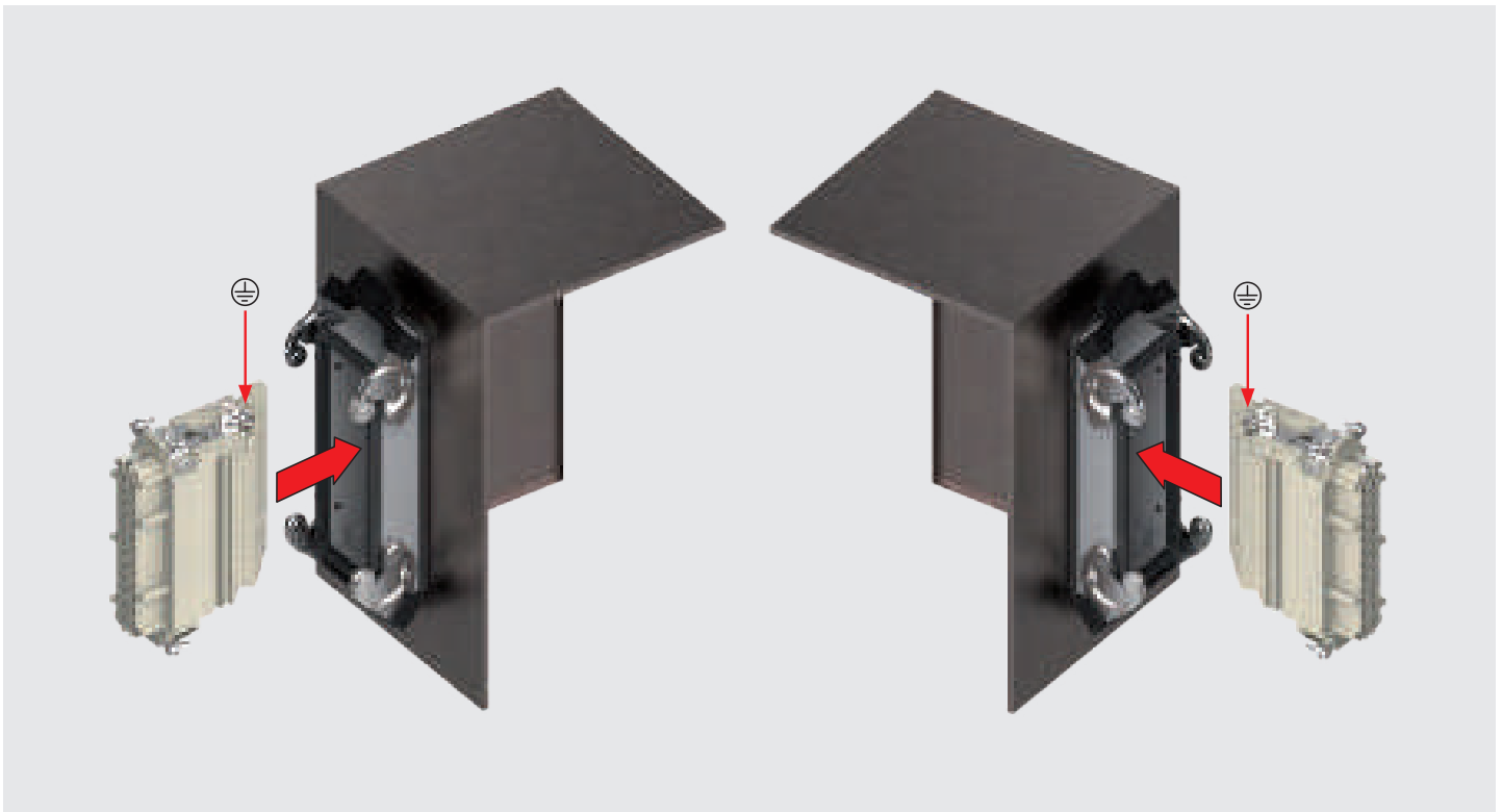
Figure 3 (left mounting)
