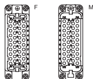
contacts side (front view)
