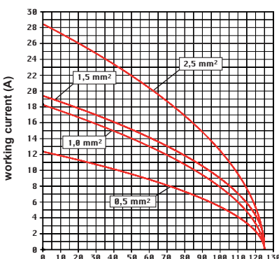
CQ 05 poles connector inserts Maximum current load derating diagram
