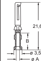
CDF and CDM contacts
