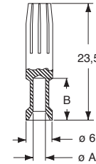
RXF2D and RXM2D contacts
