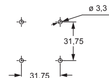
panel cut-out for enclosures
