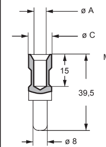
CGF and CGM
