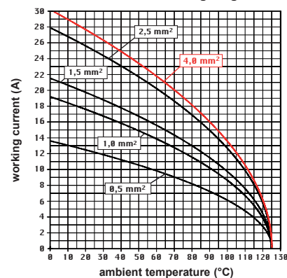
CSH 06 poles connector inserts Maximum current load derating diagram
