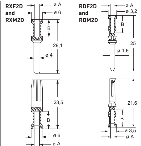
RXF2D and RXM2D contacts
