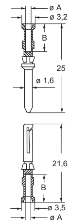
CDF and CDM contacts
