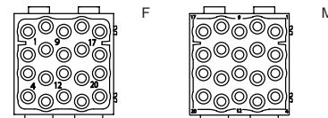
contacts side (front view) side with reference arrow ▲
