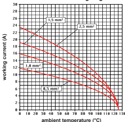
CMSH 20 poles connector inserts Maximum current load derating diagram
