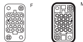
contacts side (front view)
