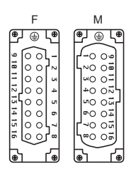
contacts side (front view)
